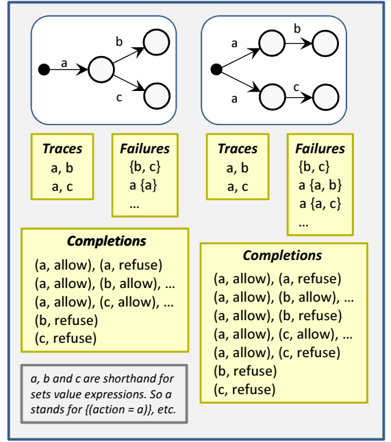
Figure 1: Traces, Failures and Completions
